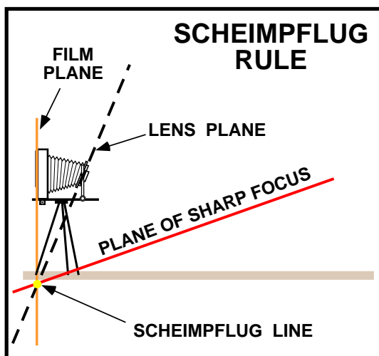
Figure 1: The Scheimpflug Rule
